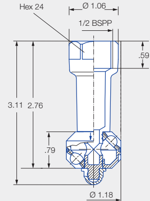
Female thread
