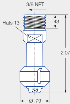
Male thread
