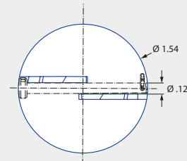
Insertion diameter of slip-on connection 2.4602 (Alloy 22)
