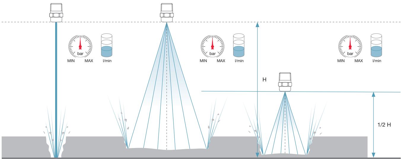
Comparison of the cleaning result of three nozzles at an identical pressure level and flow rate.
