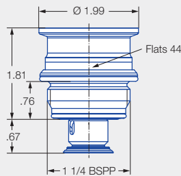
Male thread
