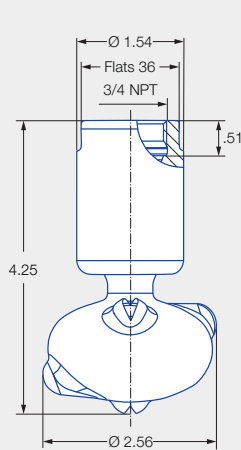
Female thread
