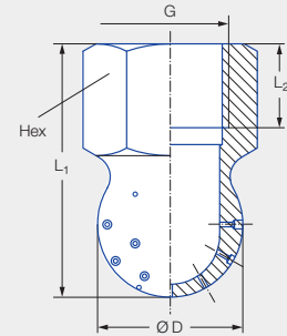
Female thread
