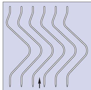
LTV 400 profile geometry
