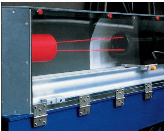
Measurement equipment: Laser-Doppler particle analyzer
